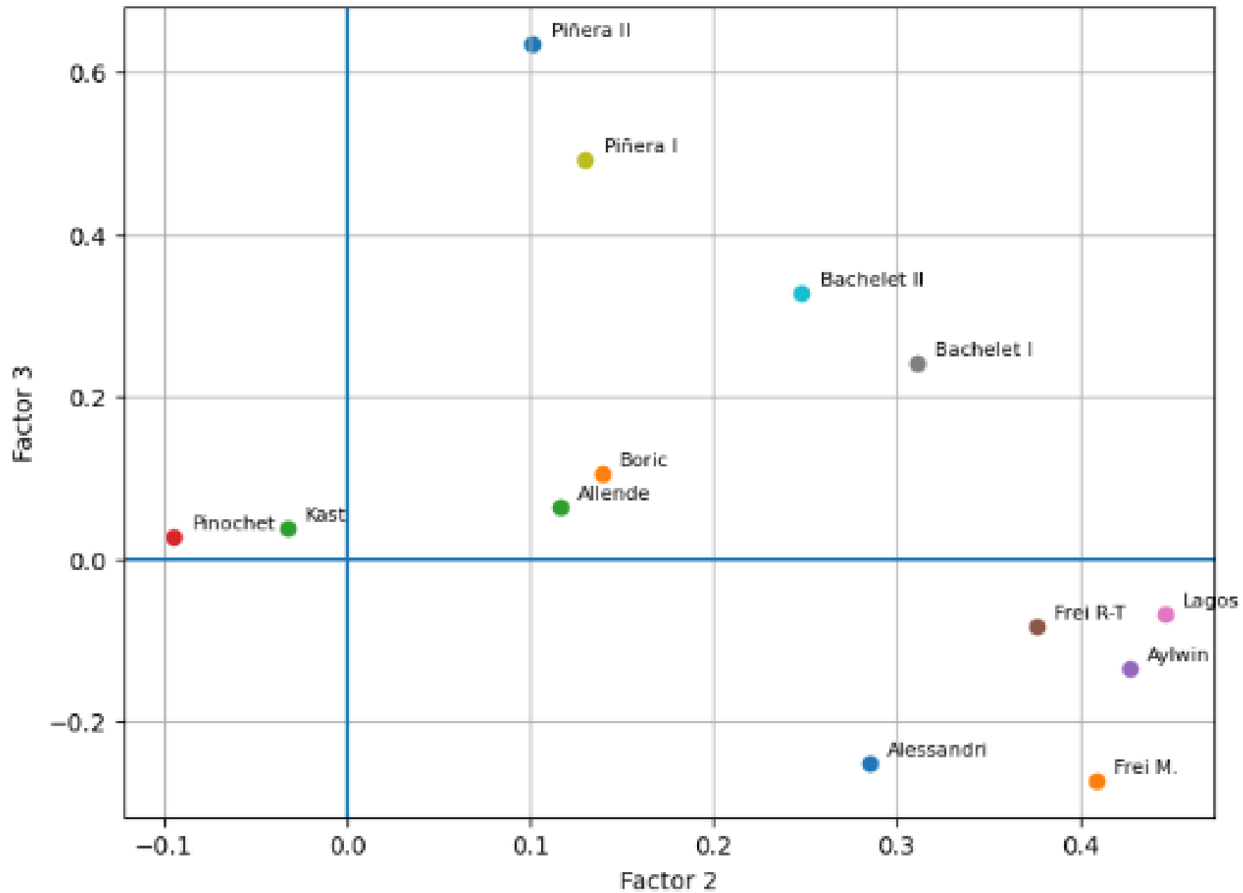
Plano Factor 2 vs Factor 3
